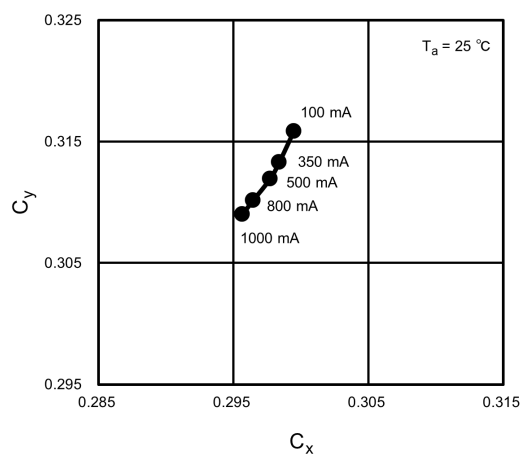
Fig. 8.4 Chromaticity - I_F
