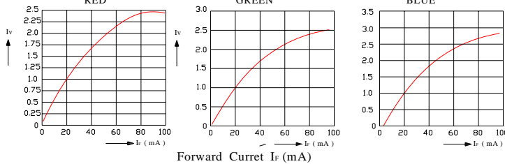
FIG.3 RELATIVE LUMINOUS INTENSITY VS. FORWARD CURRENT
