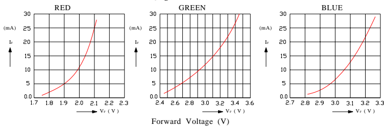
FIG.2 FORWARD CURRENT VS. FORWARD VOLTAGE
