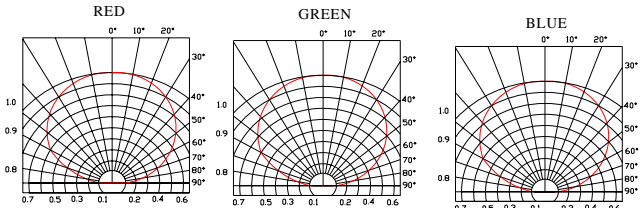
FIG.5 RADIATION DIAGRAM
