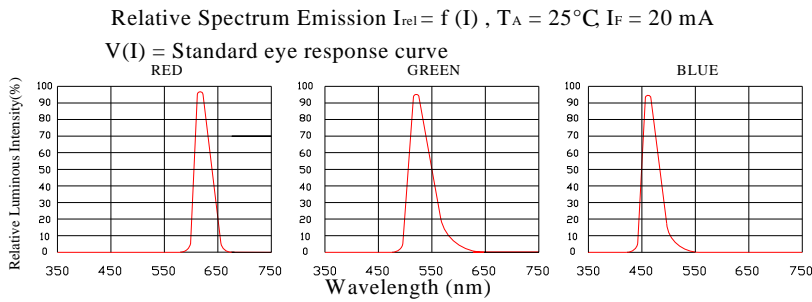
FIG.1 RELATIVE LUMINOUS INTENSITY
