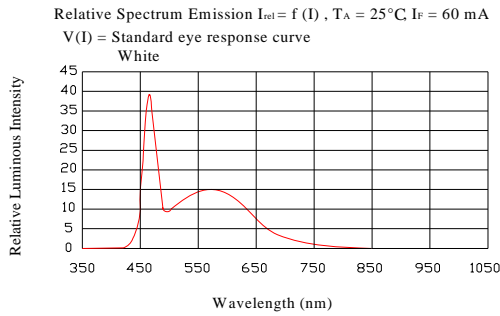
FIG.1 RELATIVE LUMINOUS INTENSITY
