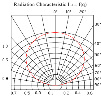
FIG.5 RADIATION DIAGRAM
