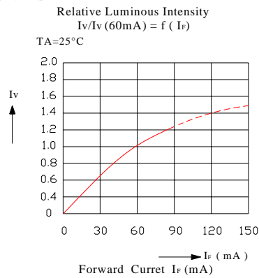
FIG.3 RELATIVE LUMINOUS INTENSITY VS. FORWARD CURRENT
